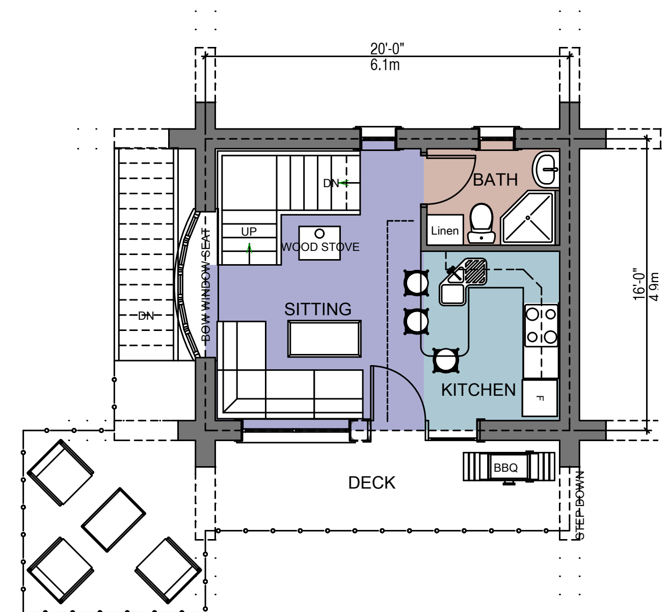
FIRST FLOOR PLAN AREA: 320 SQ.FT. / 29.7 SQ. M
