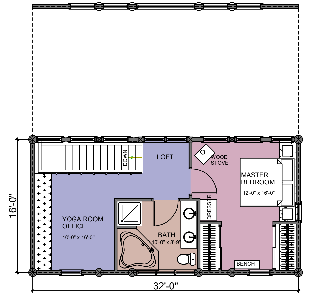
SECOND FLOOR PLAN AREA: 405 SQ. FT.
