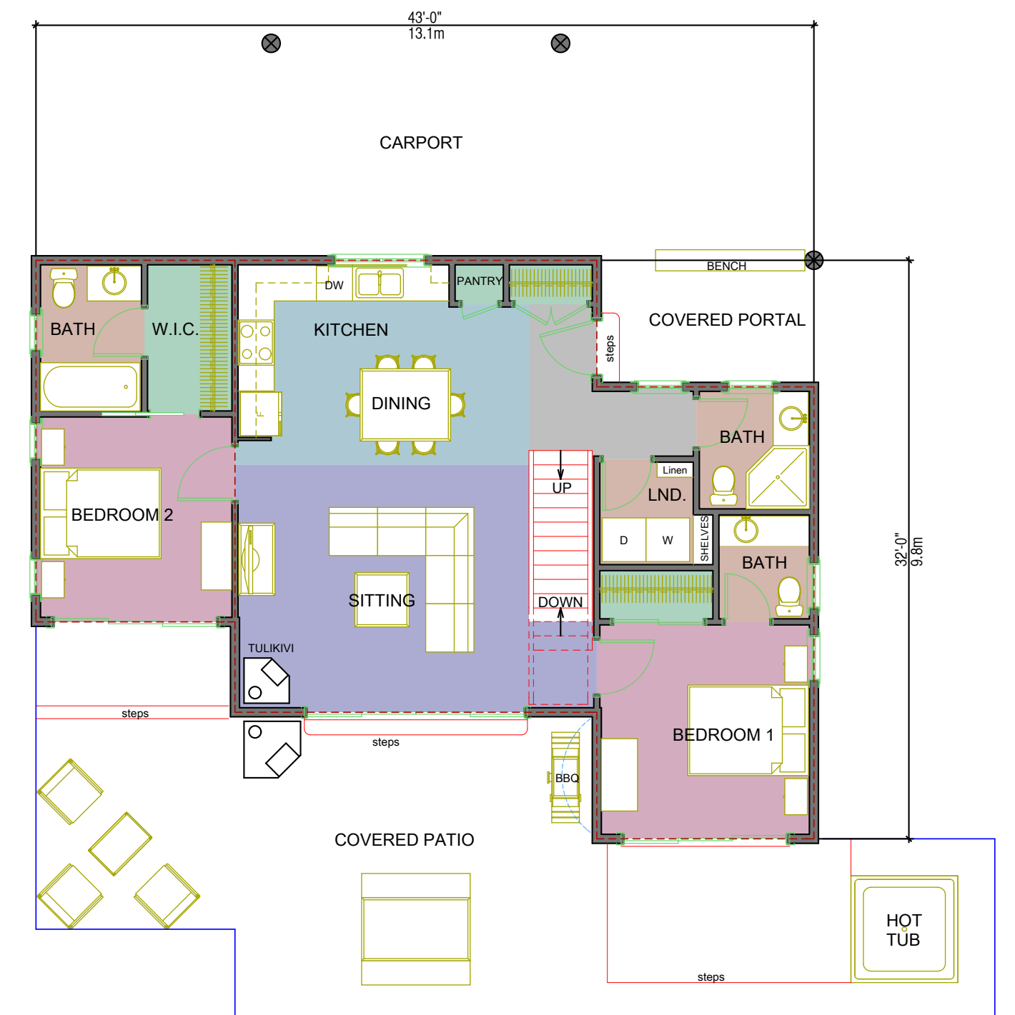
FIRST FLOOR PLAN AREA: 1058 SQ.FT. / 98.3 SQ. M
