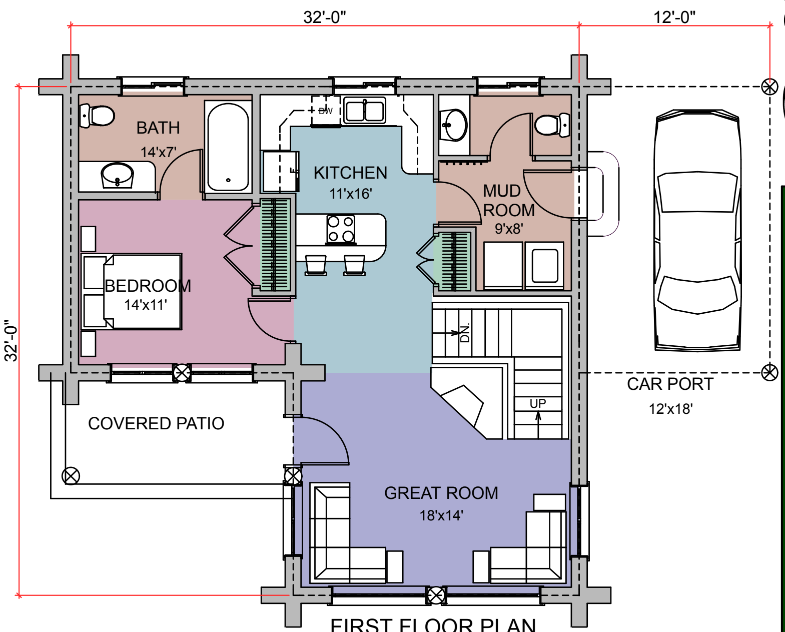
FIRST FLOOR PLAN AREA: 800 SQ.FT.
