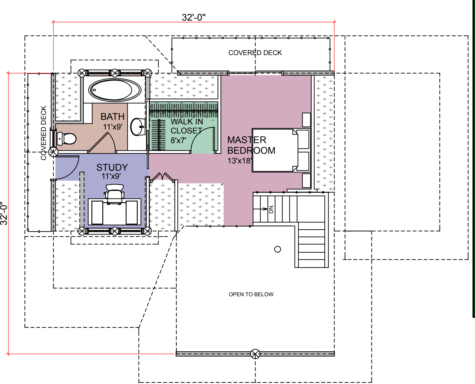
SECOND FLOOR PLAN AREA: 360 SQ. FT.
