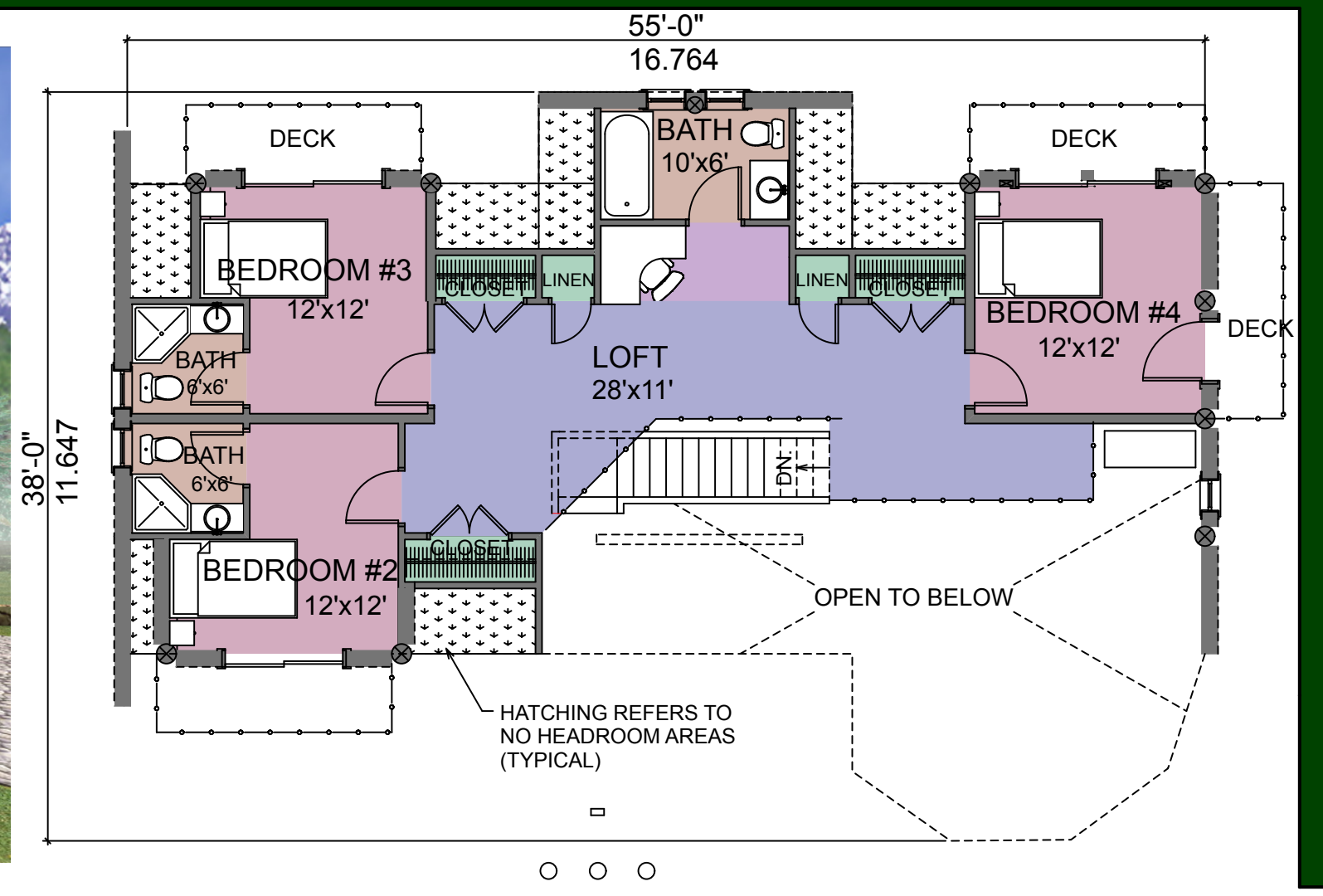
SECOND FLOOR PLAN AREA: 838 SQ. FT. 77.85m
