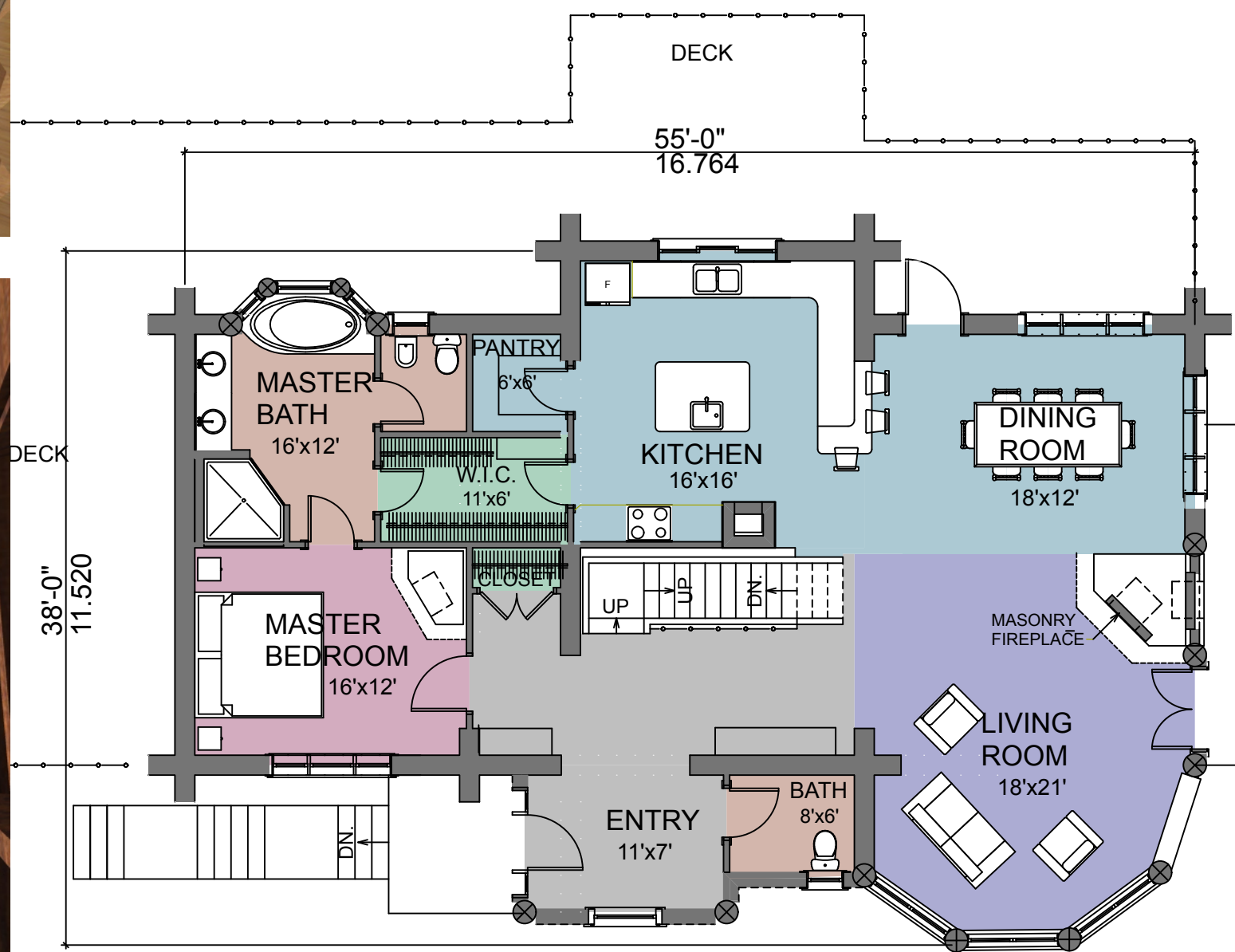
FIRST FLOOR PLAN AREA: 1552 SQ.FT. 144.19 m
