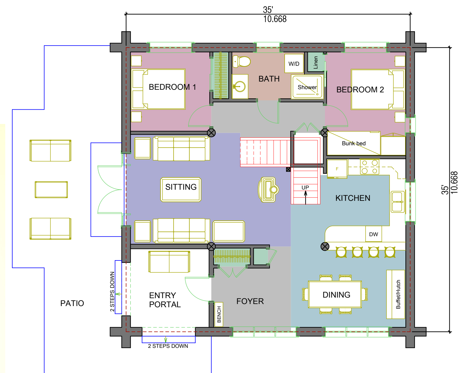
FIRST FLOOR PLAN AREA: 103.5 m 2 / 1114 SQ.FT.
