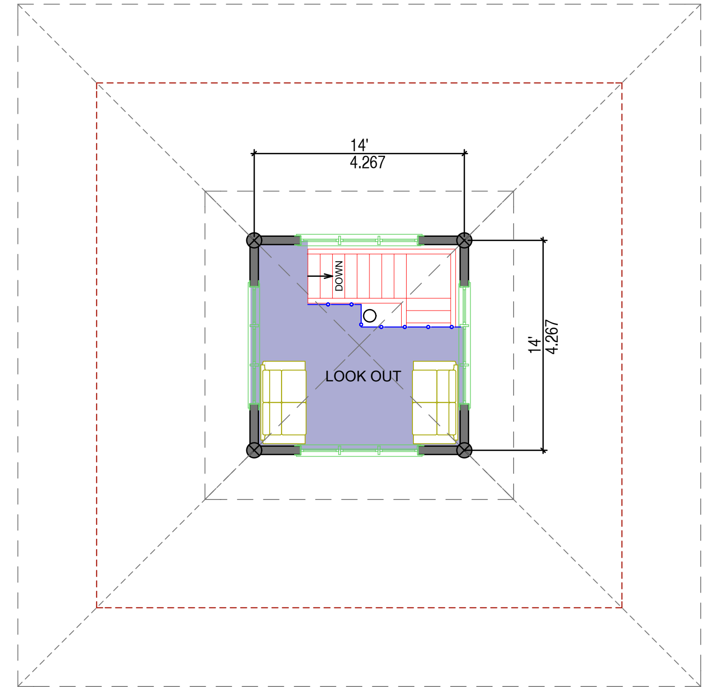
SECOND FLOOR PLAN AREA: 18.2 m 2 / 196 SQ. FT.
