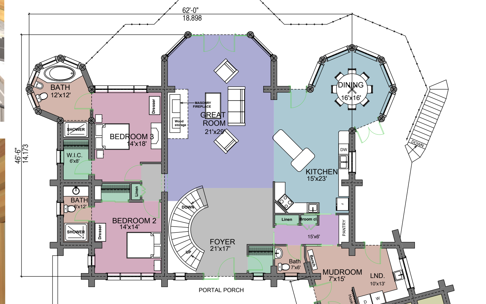
FIRST FLOOR PLAN AREA: 2614 SQ.FT. 243 SQ.M.
