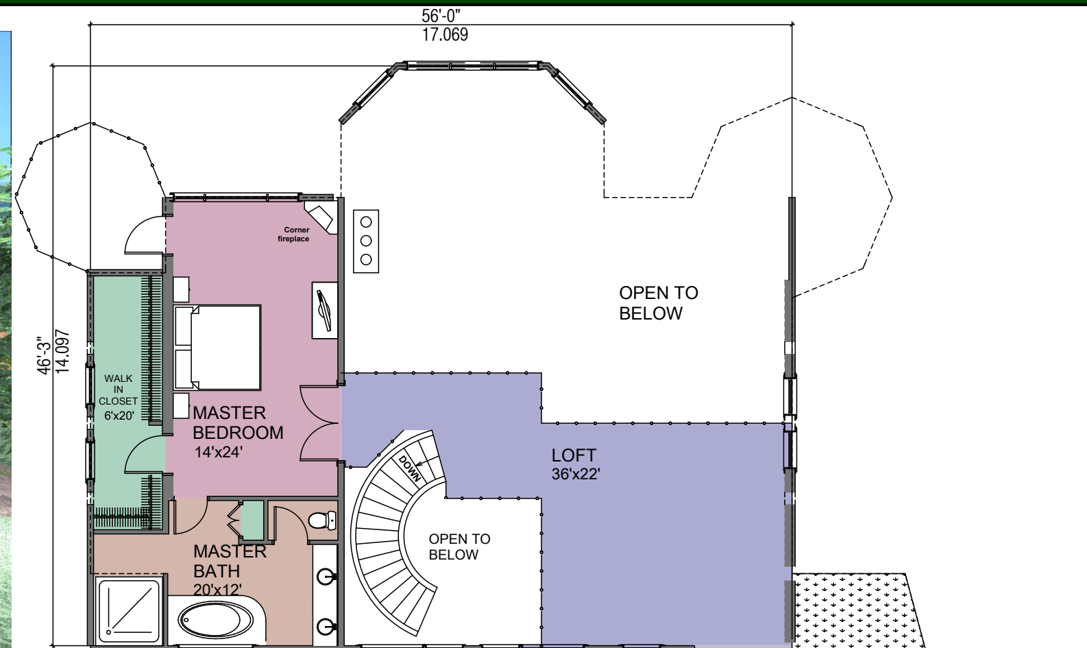
SECOND FLOOR PLAN AREA: 1621 SQ. FT. 151 SQ.M.
