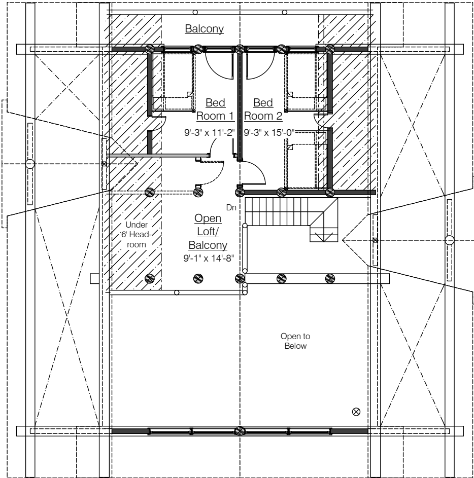
Loft Floor Plan
