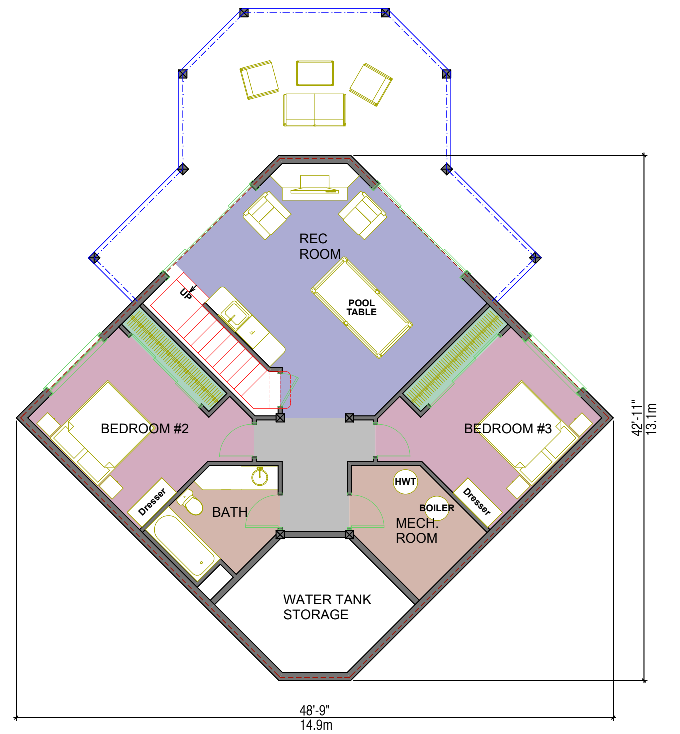
BASEMENT PLAN AREA: 1182 SQ. FT. / 109.8 SQ. M
