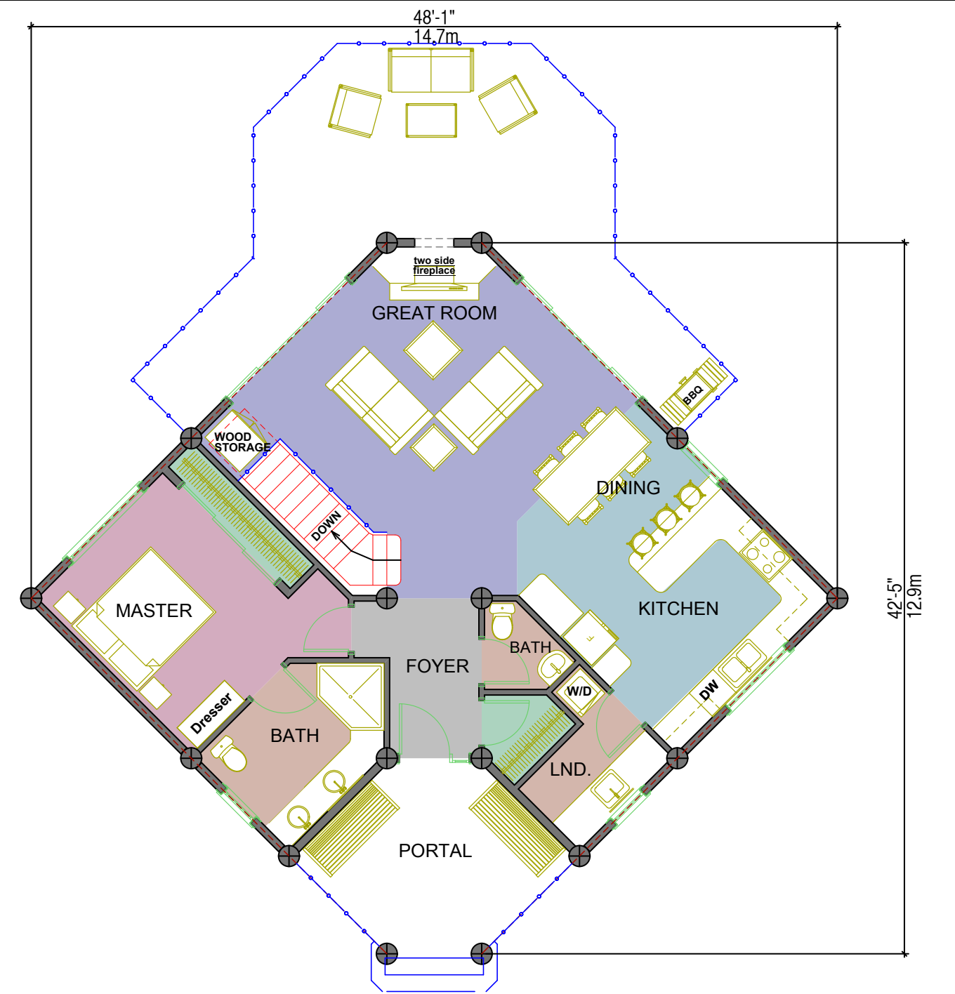
FIRST FLOOR PLAN AREA: 1039 SQ.FT. / 96.5 SQ. M
