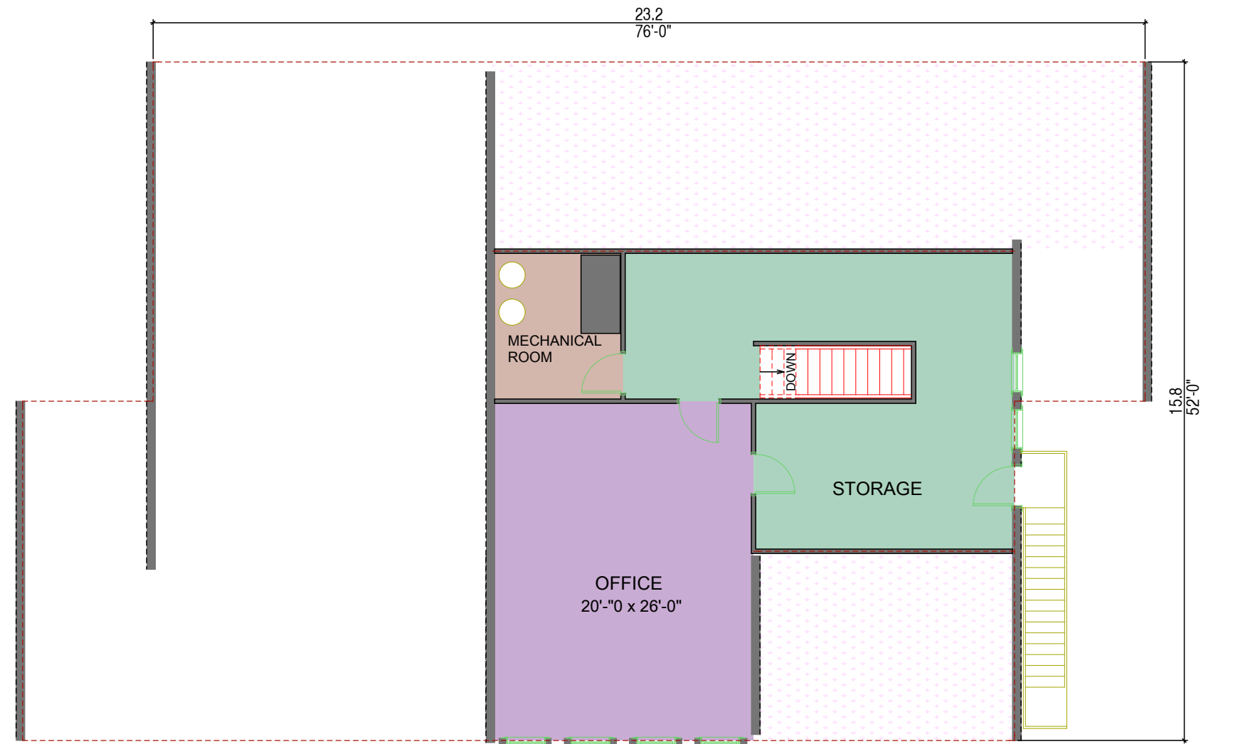
SECOND FLOOR PLAN AREA: 1210 SQ. FT. 112 SQ.M.
