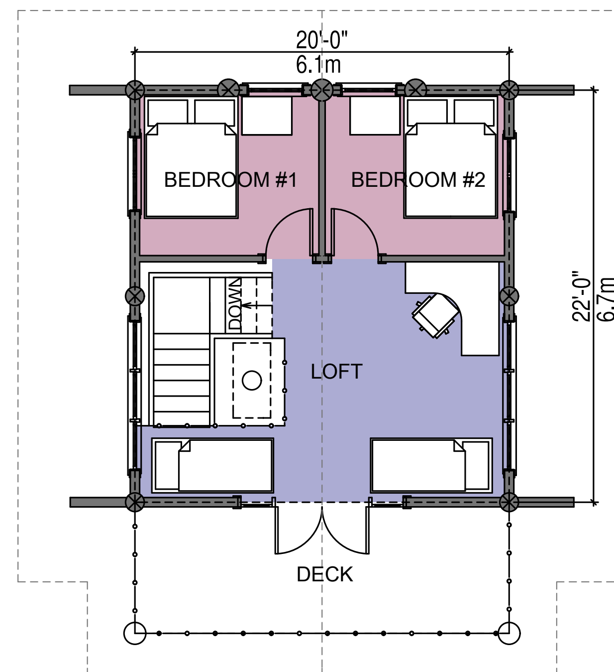
SECOND FLOOR PLAN AREA: 393 SQ. FT. / 36.5 SQ. M
