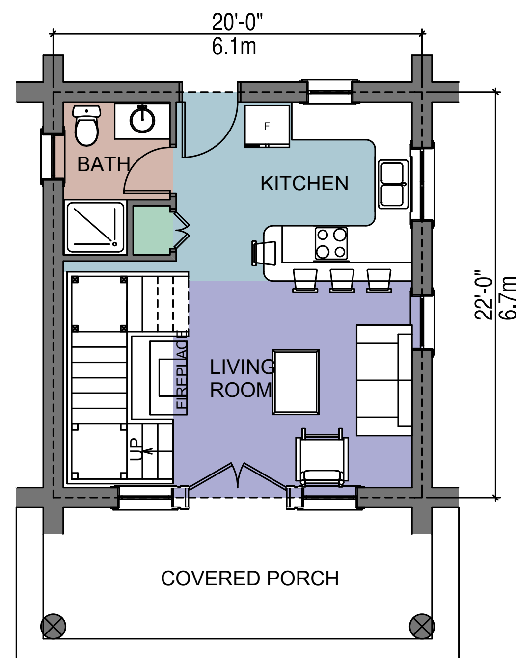
FIRST FLOOR PLAN AREA: 440 SQ. FT. / 40.9 SQ. M
