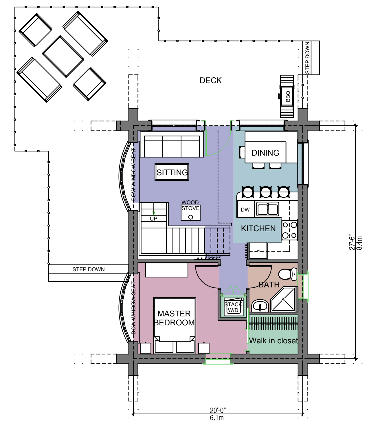
FIRST FLOOR PLAN AREA: 574 SQ. FT.
