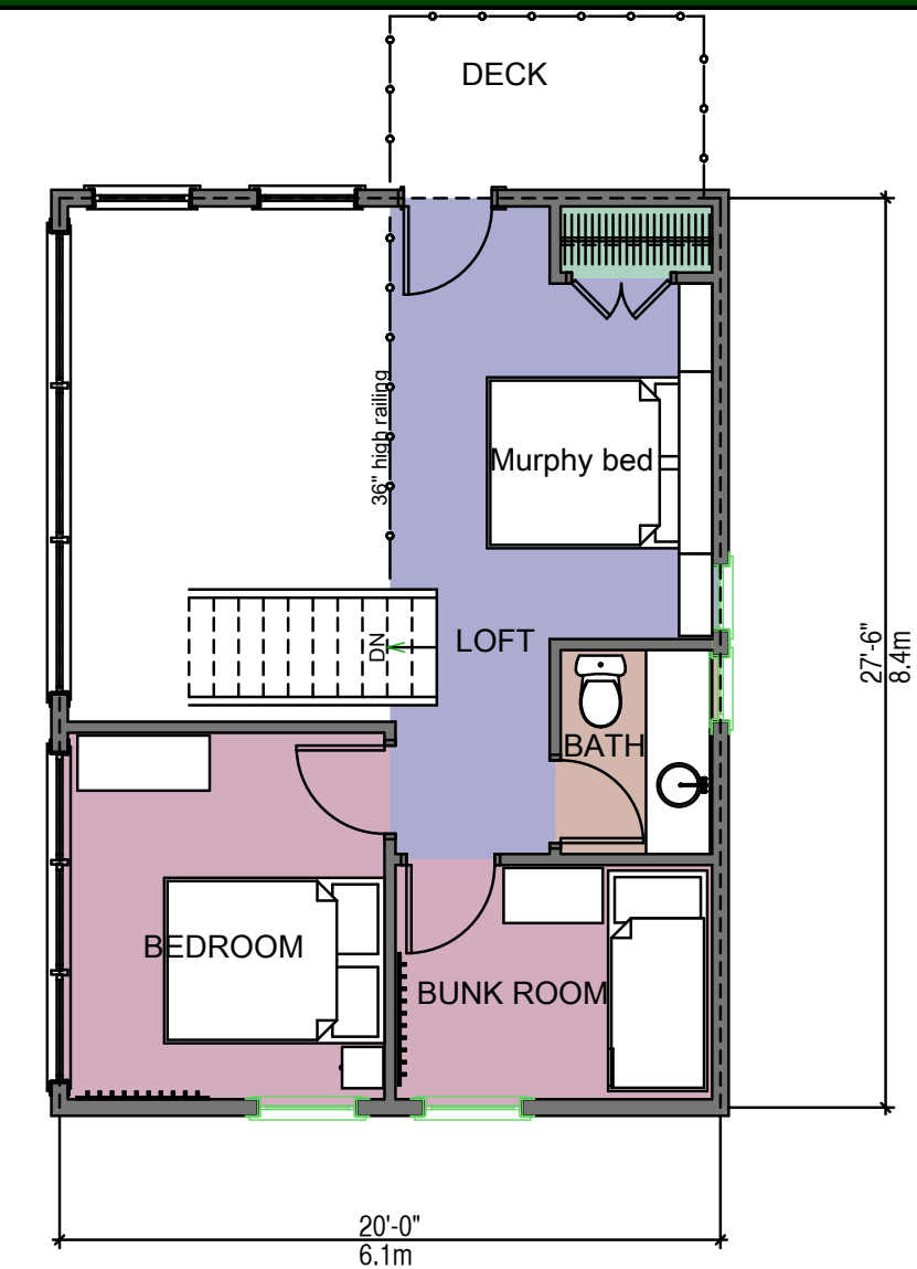
SECOND FLOOR PLAN AREA: 404 SQ. FT.
