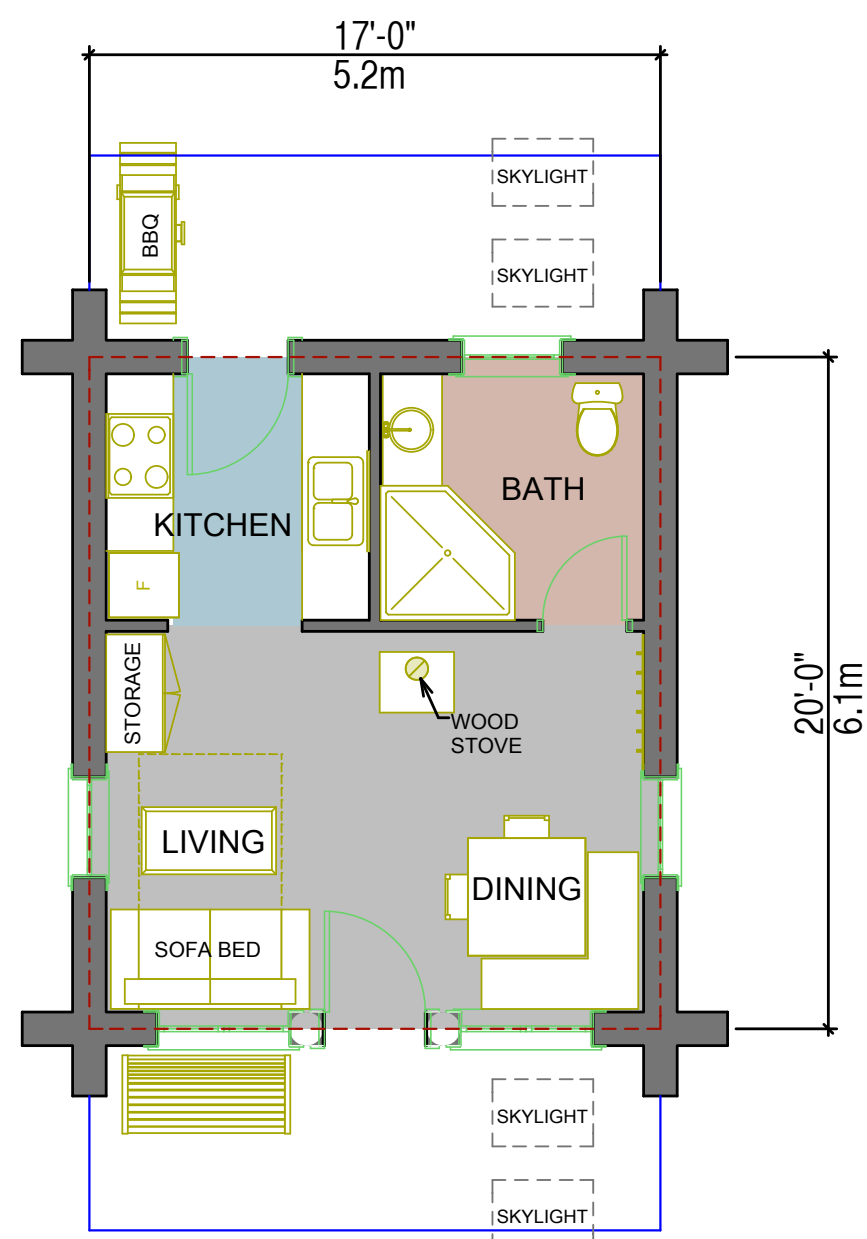
FIRST FLOOR PLAN AREA: 336 SQ.FT. / 31.2 SQ. M
